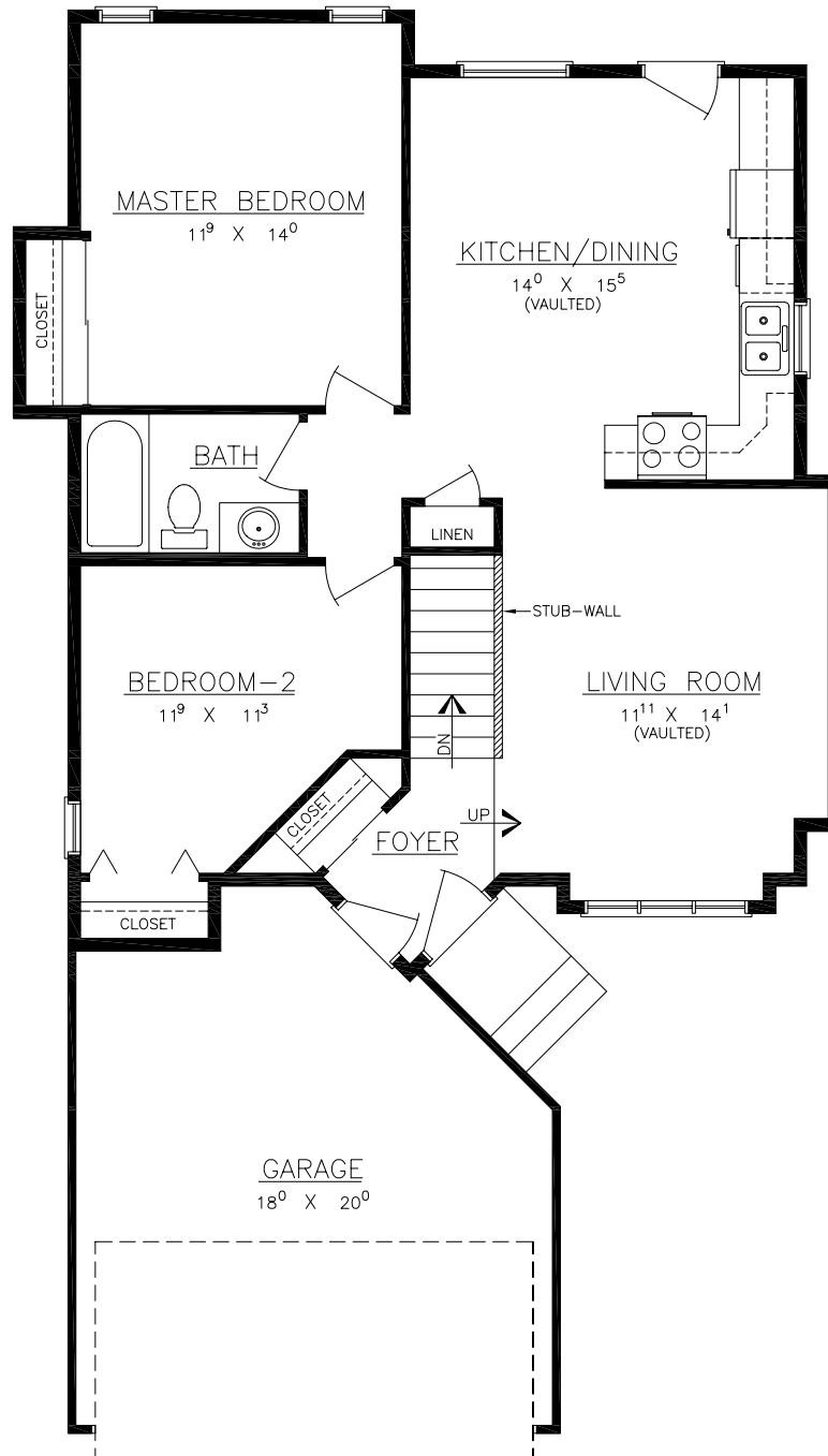
FLOOR PLAN
